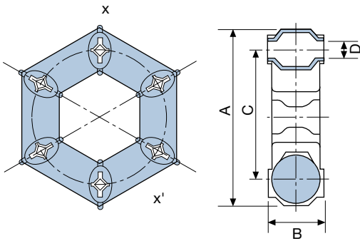
SECTION X-X'
