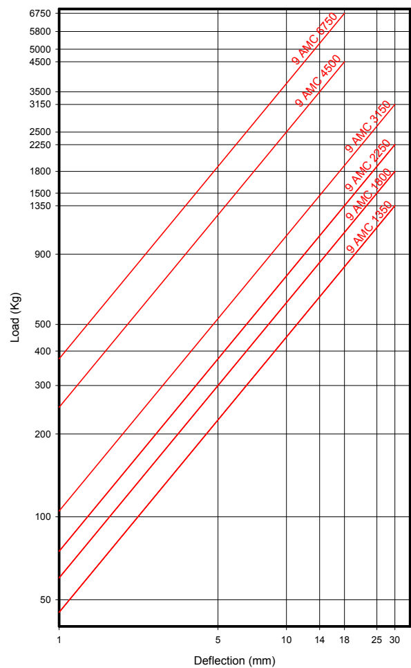
AMC LOAD DEFORMATION MECANOCAUCHO Type 9 AMC
