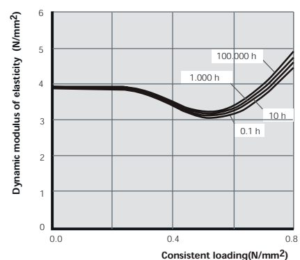
Fig.4 Dynamic modulus of elasticity at long term loading
