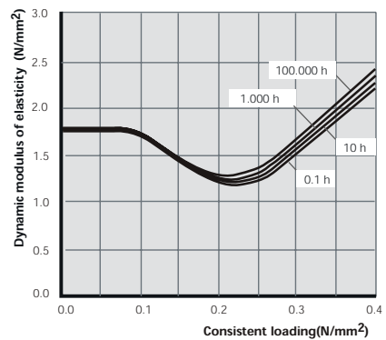
Fig.2 Dynamic modulus of elasticity at long term loading
